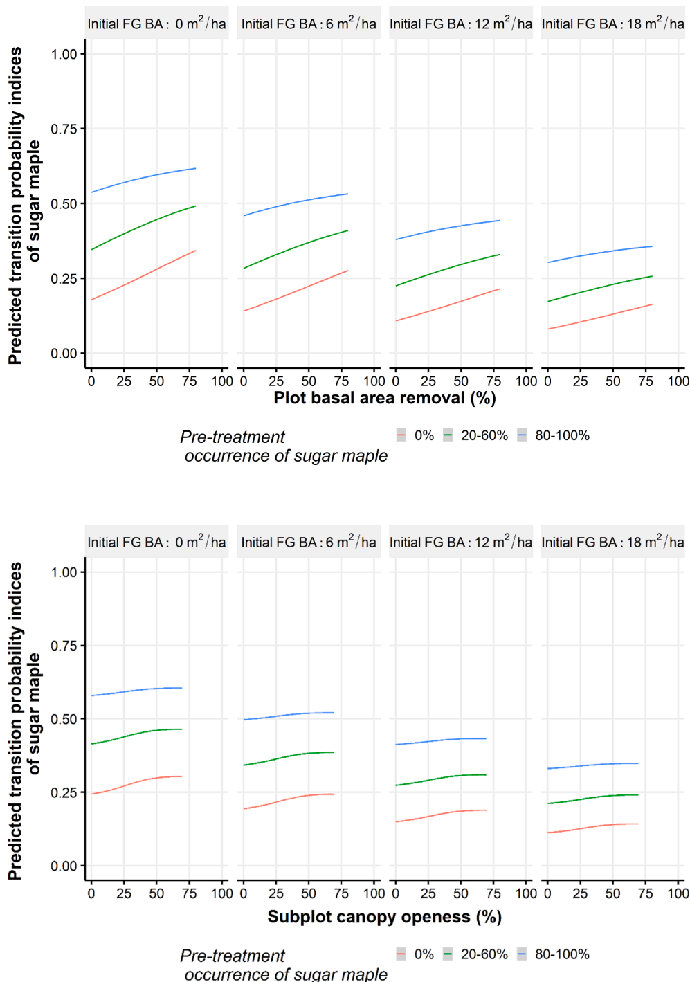
Fig. 3.5. Predictions of transition probability indices for sugar maple as a function of plot basal area removal per class of sugar maple pre-treatment occurrence in the advance seedling regeneration and initial beech basal area (FG BA). Because we predicted transition probabilities from a simulated database, no confidence intervals are presented. We divided the observed range of basal area removal (0 to 80%) into four sections and calculated the mean canopy openness for each. For a simulated basal area removal of 0 to 20%, the mean canopy openness was 8%. For a simulated basal area removal of 20 to 40%, 40 to 60% and 60 to 80%, the mean canopy openness was 10%, 15% and 27%, respectively. For every jump of 1% in basal area removal, we generated all possible combinations with the other variables.
